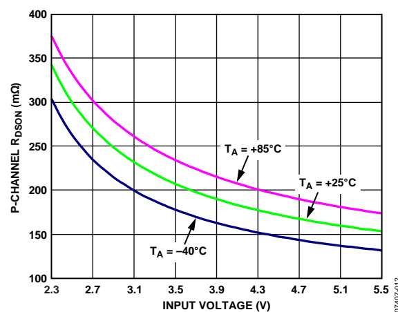
Figure 21. P-Channel Drain-Source On Resistance
