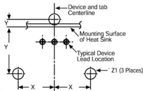
Mounting Details:
