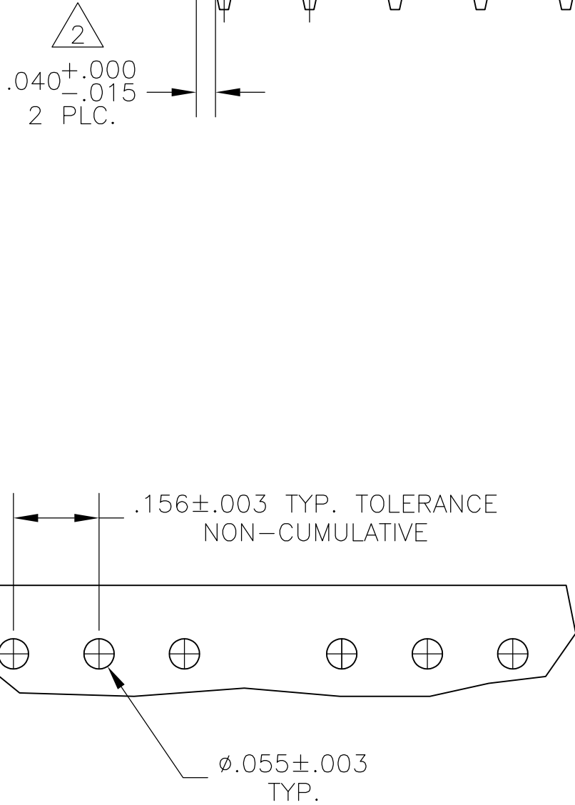
RECOMMENDED HOLE LAYOUT
