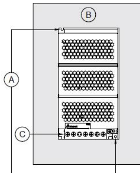
Fig. 2 Mounting Orientation
