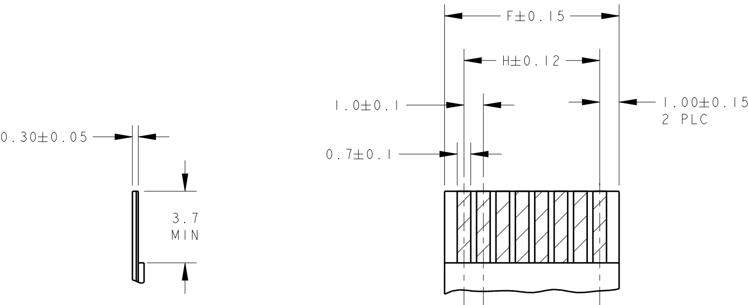
RECOMMENDED FFC/FPC
