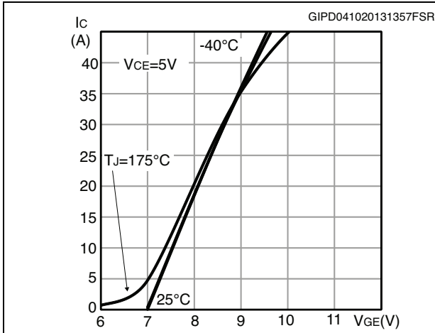
Figure 14. Transfer characteristics
