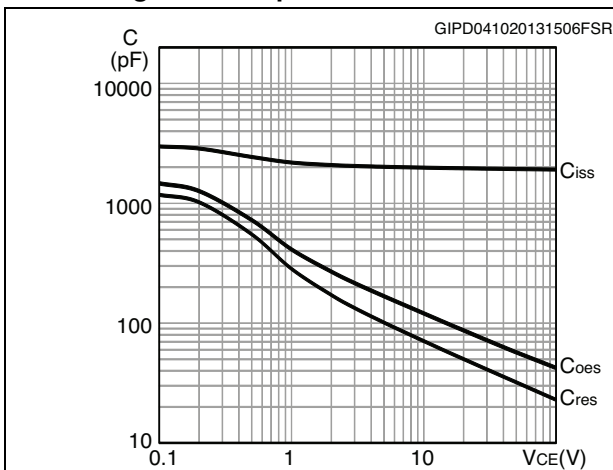
Figure 18. Capacitance variation
