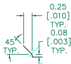
DETAIL "A" CHAMFER SCALE=15:1
