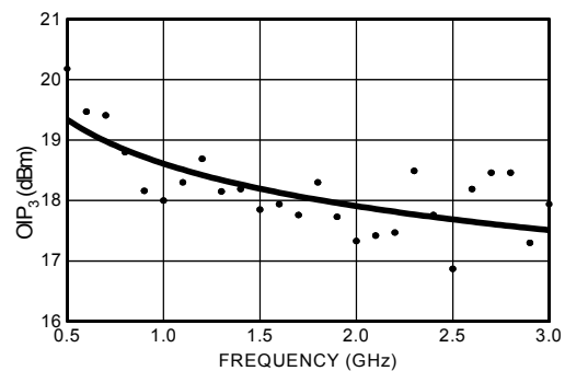
FIGURE 7. OIP3 vs FREQUENCY
