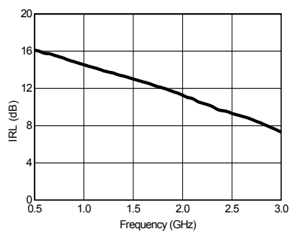
FIGURE 1. INPUT RETURN LOSS vs FREQUENCY
