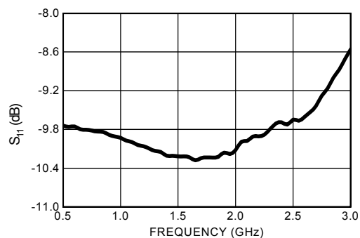
FIGURE 4. |S_{11}| vs FREQUENCY
