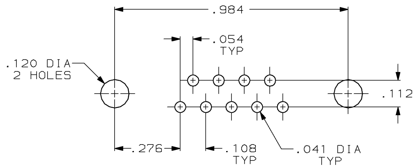
P.C. BOARD MOUNTING DIMENSIONS
