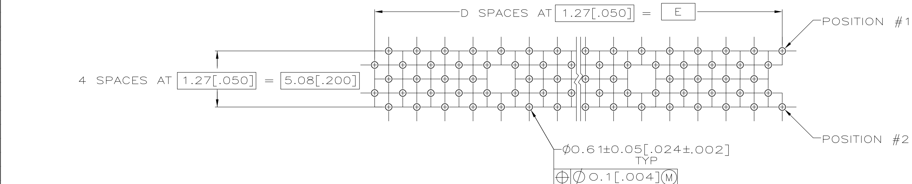
RECOMMENDED PC BOARD HOLE LAYOUT (VIEWED FROM CONNECTOR SIDE) SCALE 5:1
