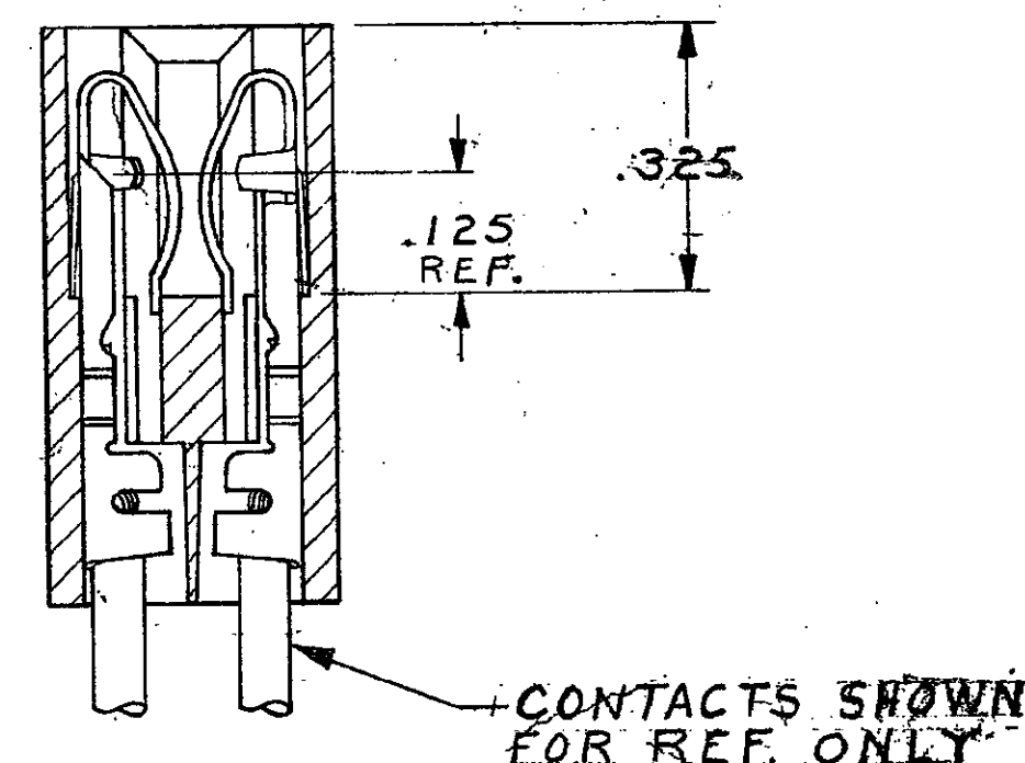
SECT. A-A
