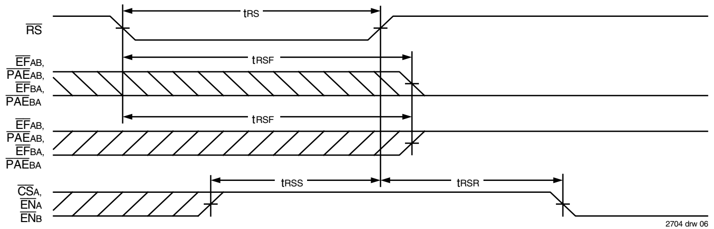
Figure 3. Reset Timing
