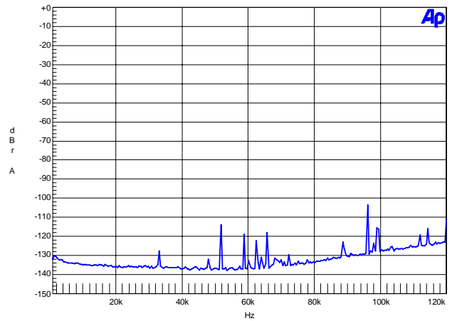
Figure 48. FFT (96 kHz Out-of-Band, No Input)
