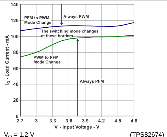
Figure 40. PFM/PWM Boundaries
