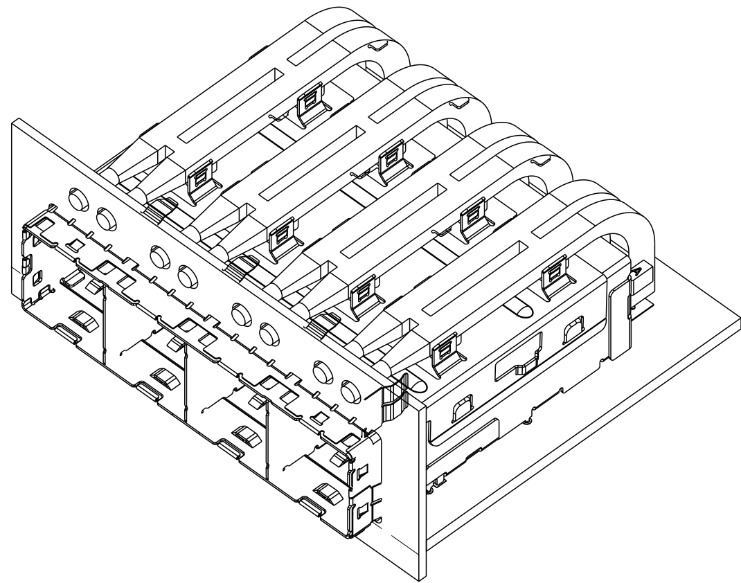
1X4 LIGHT PIPE SUB-ASSEMBLY APPLIED TO CONNECTOR 10120728-101 & 101LF SHOWN (LIGHT PIPE SUB-ASSEMBLY FINAL ASSEMBLY BY CUSTOMER)
