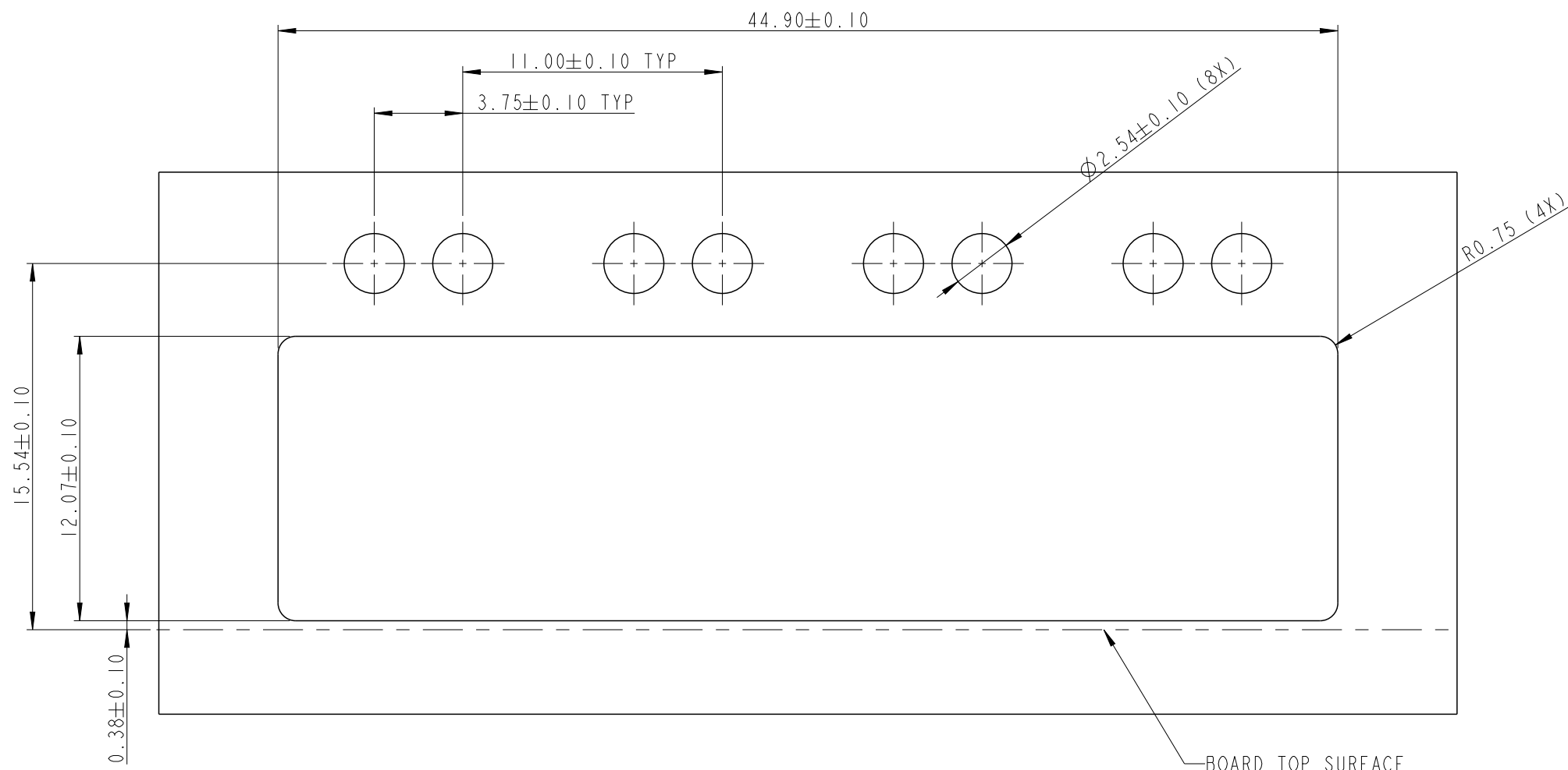
I/O BRACKET CUT OUT (BRACKET NOT SUPPLIED) SCALE 4.000
