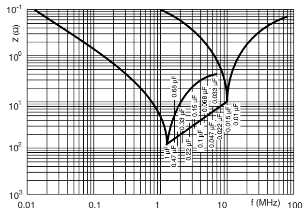
Impedance ( Z ) as a function of frequency ( f ) at T_a = 20^{\circ}C (average) Measurement with length 6 mm
