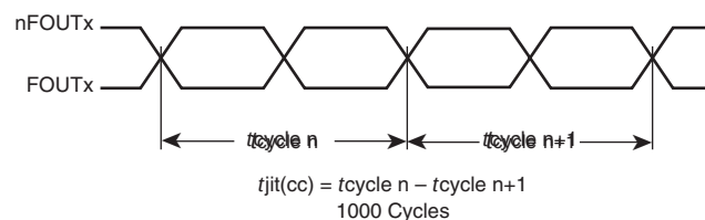
CYCLE-TO-CYCLE JITTER
