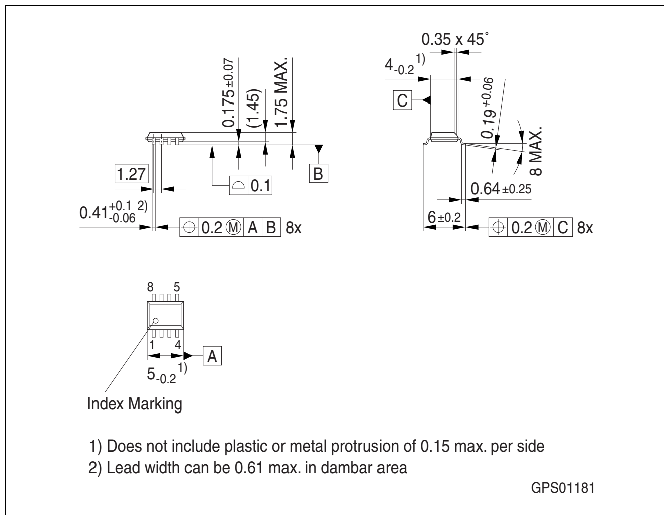
Figure 11 PG-DSO-8
