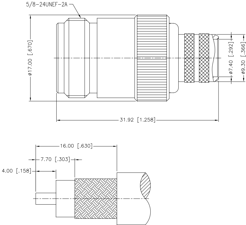
RECOMMENDED CABLE STRIPPING DIM'S
