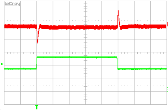
Figure 9. Output voltage response to load current step (3.5 A–5.25 A–3.5 A) at V_{in} = 48 V. Top trace: output voltage (100 mV/div.). Bottom trace: load current (2 A/div.). Current slew rate: 1 A/ \mu s. C_o = 100 \mu F Tantalum + 1 \mu F ceramic. Time scale: 0.2 ms/div.
