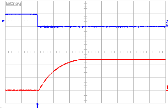
Figure 7. Turn-on transient at full rated load current (resistive) plus 3,300 \mu F at V_{in} = 48 V, triggered via ON/OFF pin. Top trace: ON/OFF signal (5 V/div.). Bottom trace: Output voltage (5 V/div.). Time scale: 2 ms/div.
