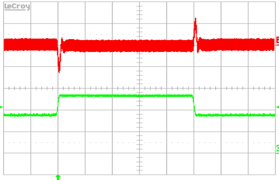
Figure 8. Output voltage response to load current step (3.5 A–5.25 A–3.5 A) at V_{in} = 48 V. Top trace: output voltage (100 mV/div.). Bottom trace: load current (2 A/div.). Current slew rate: 0.1 A/ \mu s. C_o = 1 \mu F ceramic + 10 \mu F tantalum. Time scale: 0.2 ms/div.
