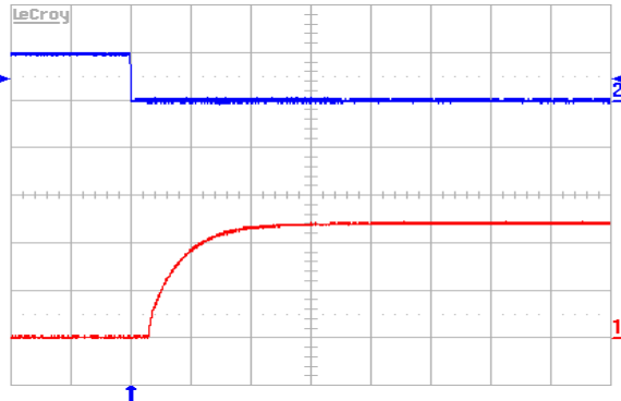
Figure 6. Turn-on transient at full rated load current (resistive) with no output capacitor at V_{in} = 48 V, triggered via ON/OFF pin. Top trace: ON/OFF signal (5 V/div.). Bottom trace: Output voltage (5 V/div.). Time scale: 2 ms/div.
