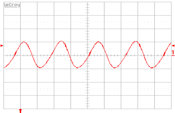
Figure 10. Output voltage ripple (10 mV/div.) at full rated load current into a resistive load with C_o = 10 \mu F tantalum + 1 \mu F ceramic and V_{in} = 48 V. Time scale: 1 \mu s/div.
