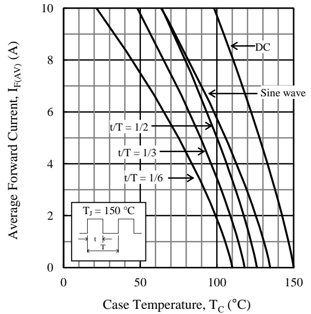
Figure 2. Typical Characteristics: I_{F(AV)} vs. T_C ( V_R = 400\text{ V} )
