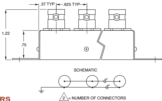
ADAPTERS MULTIPLE PARALLEL NETWORK 50Ω MPN-△/BNC 50Ω MPN-△/TNC Contact the factory for more information.
