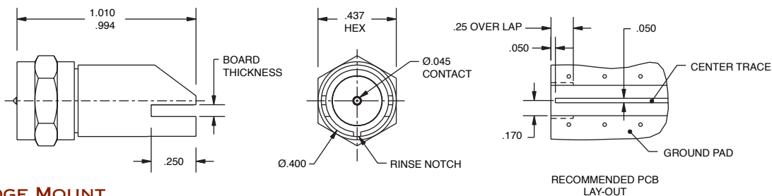
CIRCUIT BOARD EDGE MOUNT "F" STYLE MALE PLUG CBPLE130-1, -2, or -3
