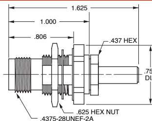
BULKHEAD CABLE JACK WRENCH CRIMP 50Ω BJ49-1 75Ω UBJ49-1 Mounting Hole: D3.218 / D2.218 (Cable Groups 6, 6E, 51, 52)
