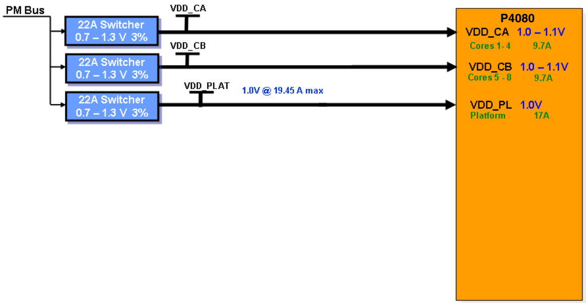
Figure 18. P4080DS Power Architecture for P4080 Part 1 of 3
