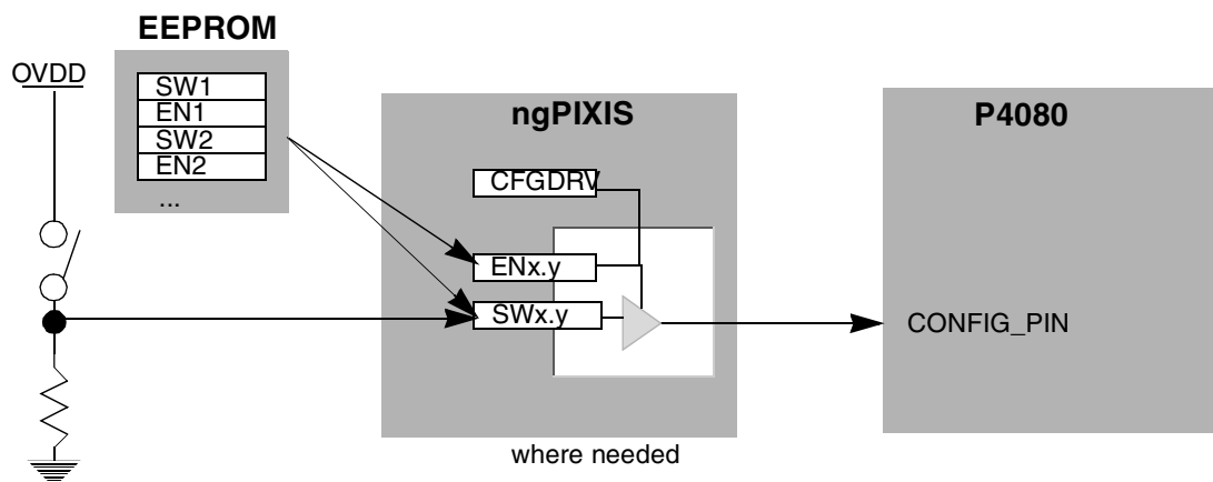
Figure 25. Configuration Logic
