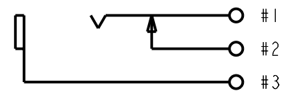
SCHEMATIC CIRCUIT
