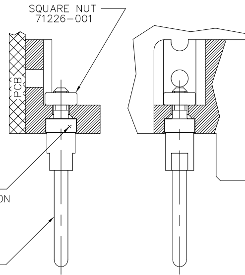
ASSEMBLED GUIDE PIN
