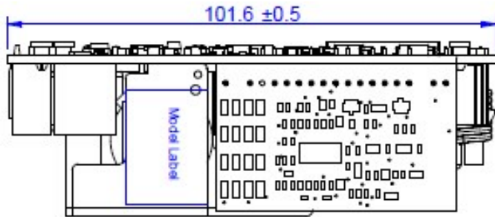
Figure 16. Side view 2
