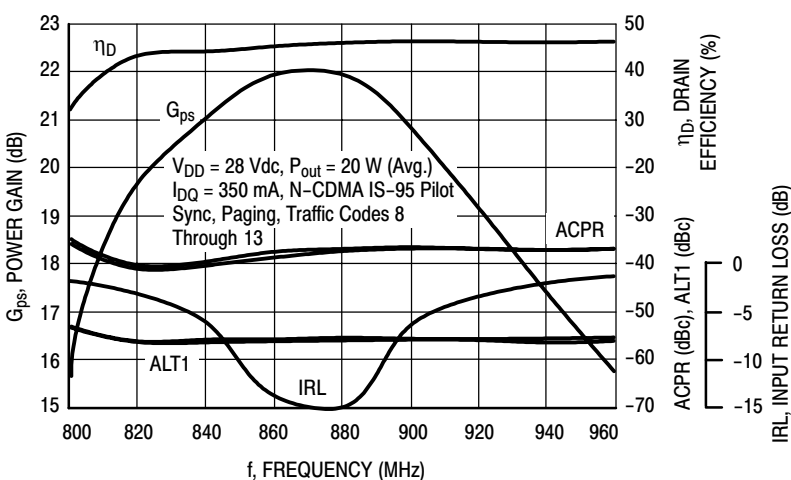
Figure 4. Single-Carrier N-CDMA Broadband Performance @ P_{out} = 20 Watts Avg.
