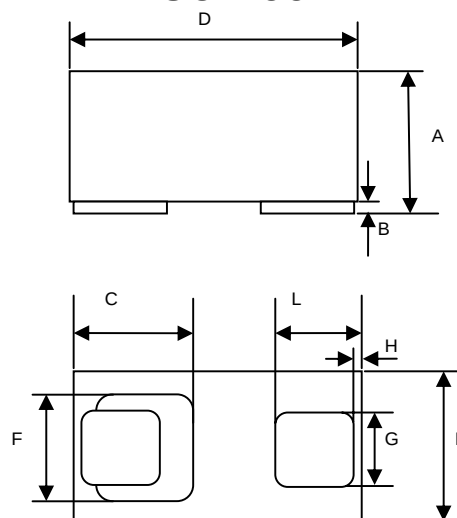
SOD-882
