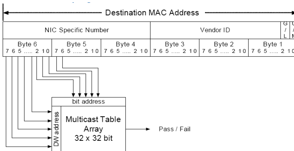
Figure 9. Multicast Table Array Algorithm
