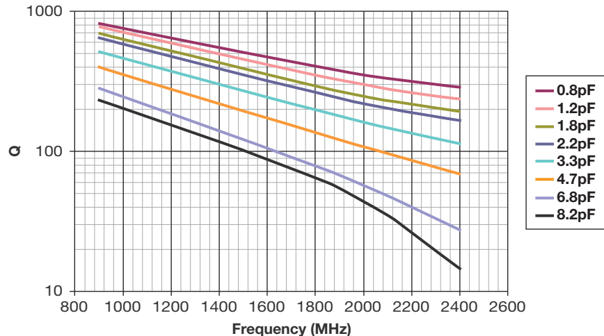
Accu-P® 0805 Typical Q vs Frequency
