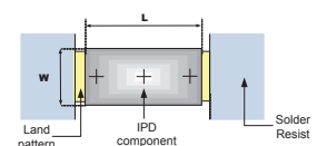
(0805 PCB footprint)
