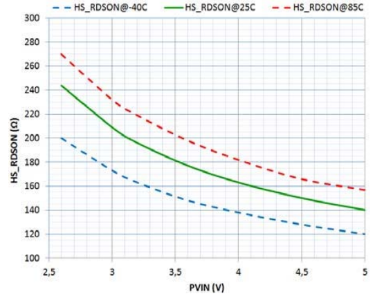
Figure 14. High-Side PMOS R_{DS(on)} vs. PV_{IN} and Temperature
