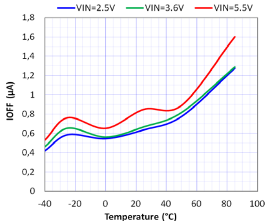
Figure 6. Shutdown Current vs Temperature ( T_A ) ( EN = \text{Low} , V_{CON} = 0\text{ V} )
