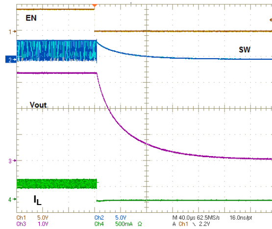
Figure 48. Power-down Transient Response PV_{IN} = 3.7\text{ V} , V_{out} = 3.4\text{ V} , R_L = 10\text{ }\Omega
