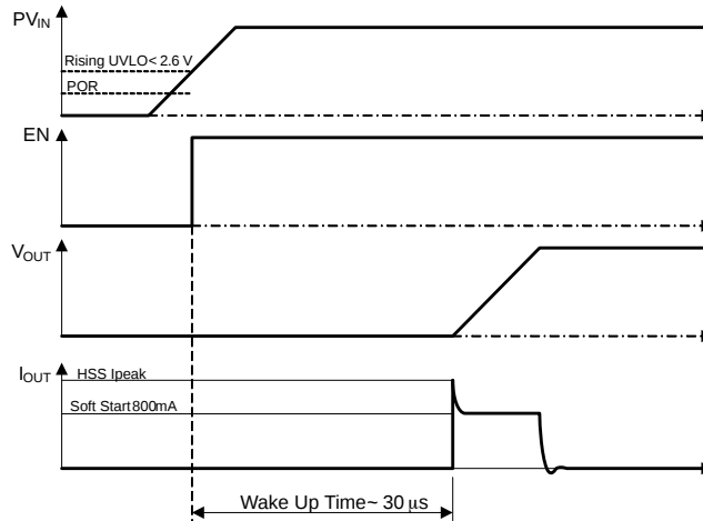
Figure 49. Power-Up Sequence
