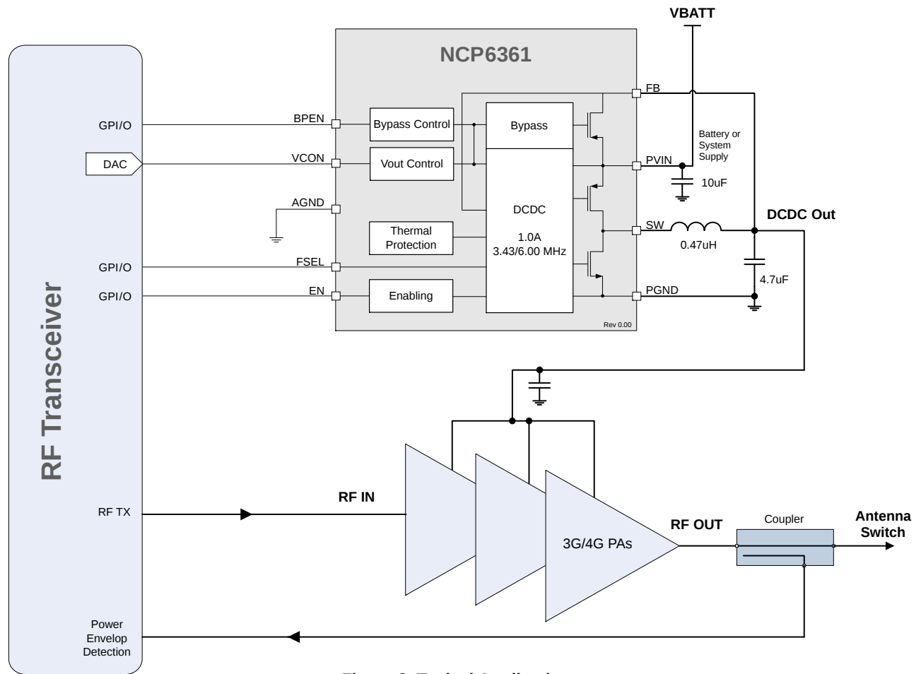
Figure 2. Typical Application
