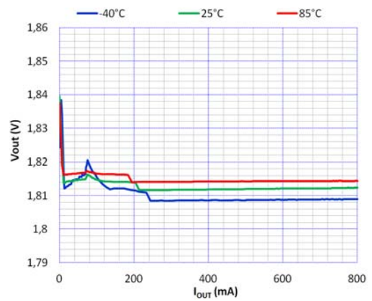
Figure 31. V_{OUT} Accuracy vs Output Current vs Temperature PV_{IN} = 3.6\text{ V} , F_{SW} = 6\text{ MHz} , V_{OUT} = 1.8\text{ V}
