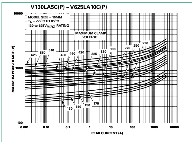
Figure 3. Maximum Clamping Voltage for 10mm Parts
