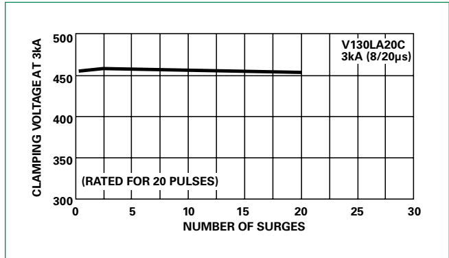
Figure 13 & 14. Typical Repetitive Surge Current Capability of C-III Series MOVs
