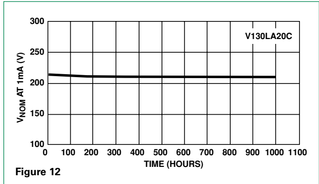
Figure 12. High Temperature Operating Life 125°C for 1000 Hours at Rated Bias
