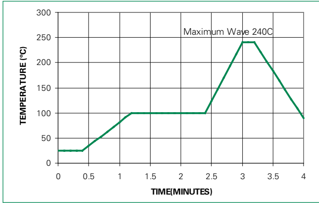
Figure 10. Non Lead-free Profile
