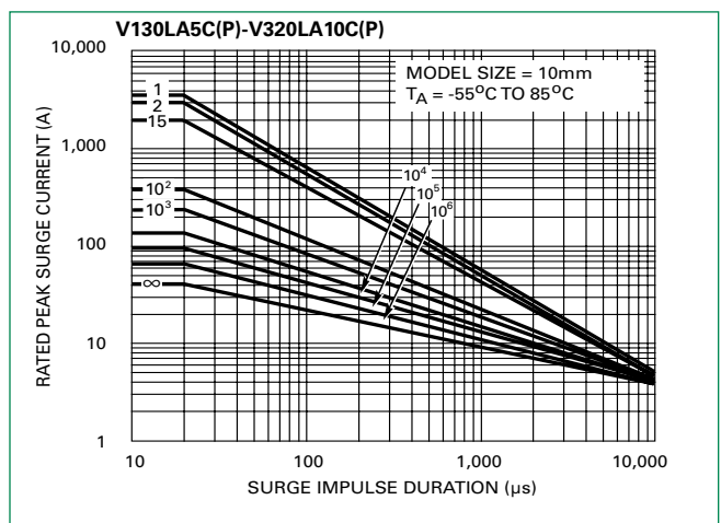
Figure 4. Repetitive Surge Capability for 10mm Parts
