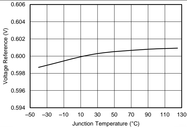
Figure 13. Voltage Reference vs Temperature
