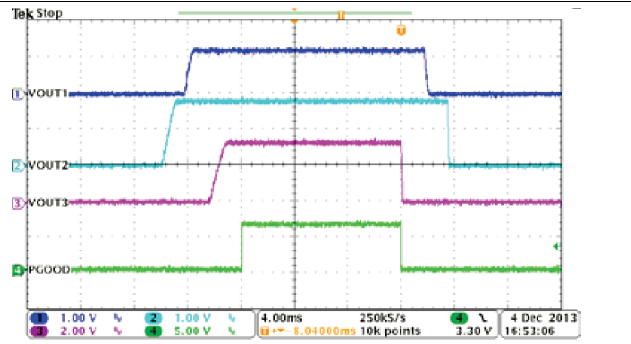
Figure 58. Automatic Power Sequencing, MODE = EN1 = HIGH, EN2 = LOW
