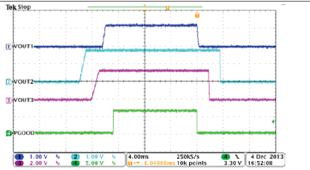
Figure 56. Automatic Power Sequencing, MODE = EN1 = EN2 = HIGH
