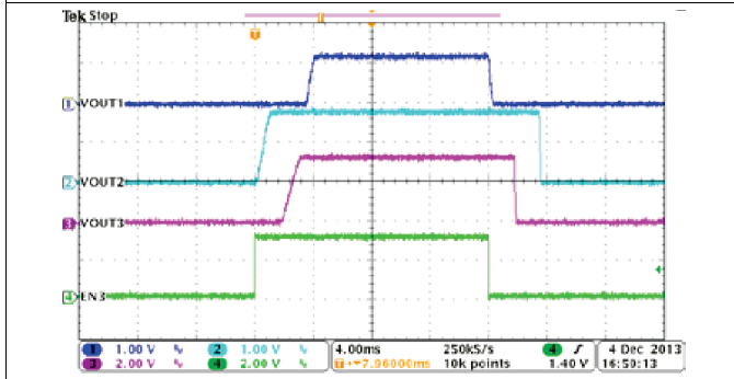
Figure 55. Automatic Power Sequencing, MODE = EN1 = EN2 = HIGH
