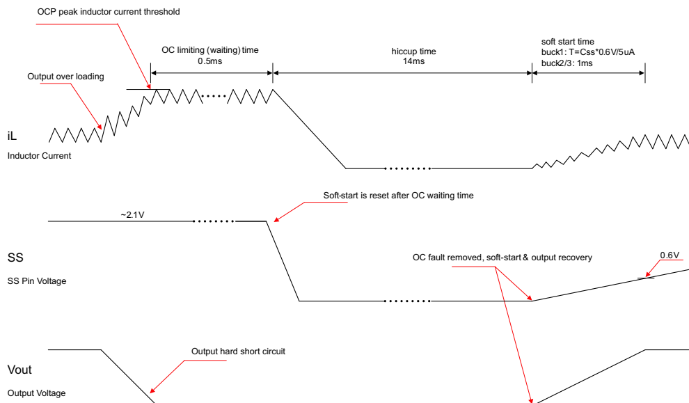
Figure 29. Overcurrent Protection
