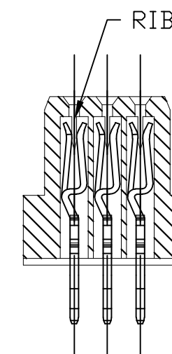
SECTION A-A SCALE: 2:1 (POWER CROWNS OMITTED FOR CLARITY)
