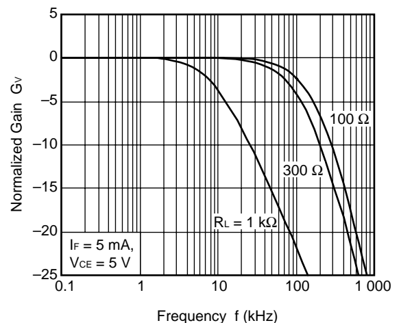
FREQUENCY RESPONSE
