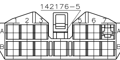
VERSION: POLARIZATIONLESS (sans detrompage) (VIEW F)
