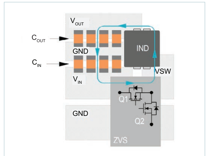
Figure 66 — Recommended component placement and metal routing
