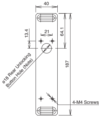
Drilling Rear Unlocking Button Hole
