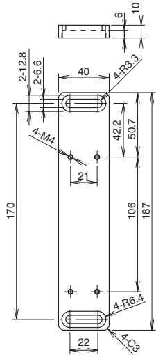
Mounting Plate (HS9Z-SP51)
