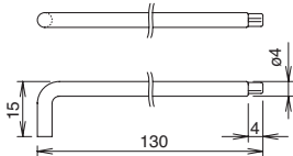
Manual Unlocking Key (Metal) (HS9Z-T3)
