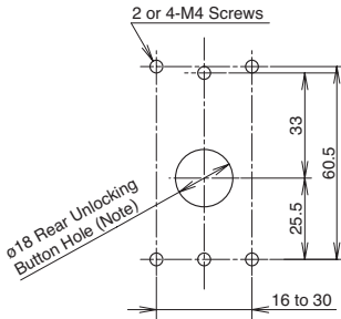
Rear Unlocking Button Kit Mounting Hole Layout
