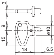
Manual Unlocking Key (plastic)
