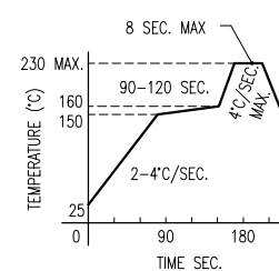
REFLOW PROFILE
