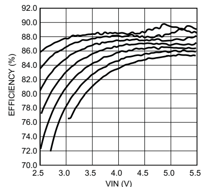
L = 10 \mu\text{H} 20 mA/String f_{SW} = 1\text{ MHz} Top To Bottom: 2x4, 2x5, 2x6, 2x7, 2x8, 2x9, 2x10 (LEDs)
