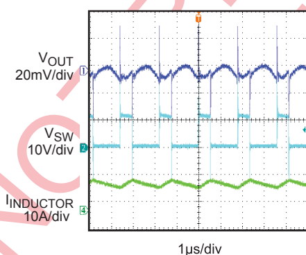
Output Ripple Voltage I_{OUT}=10A
