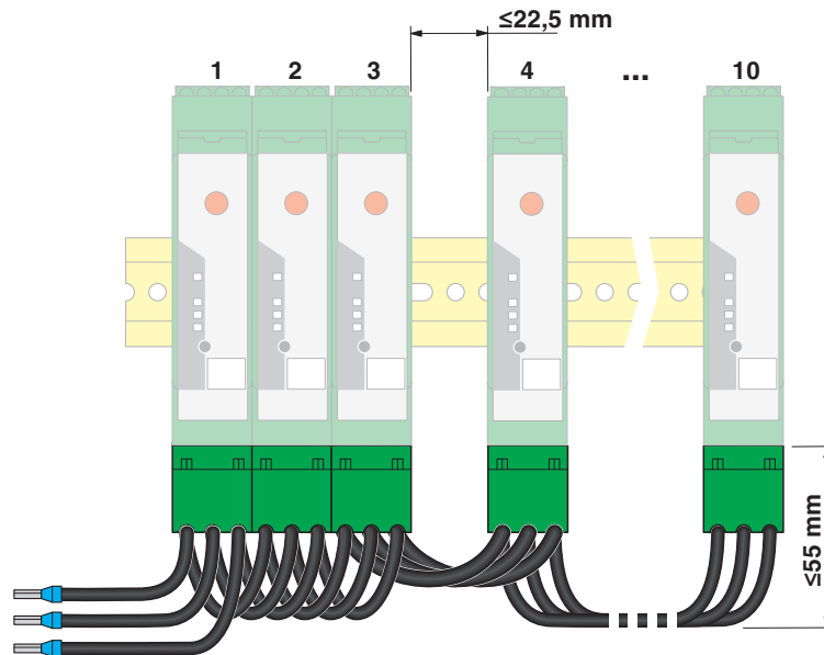
Application drawing
