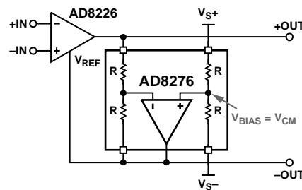
Figure 47. Differential Output With Supply Tracking on Common-Mode Voltage Reference
