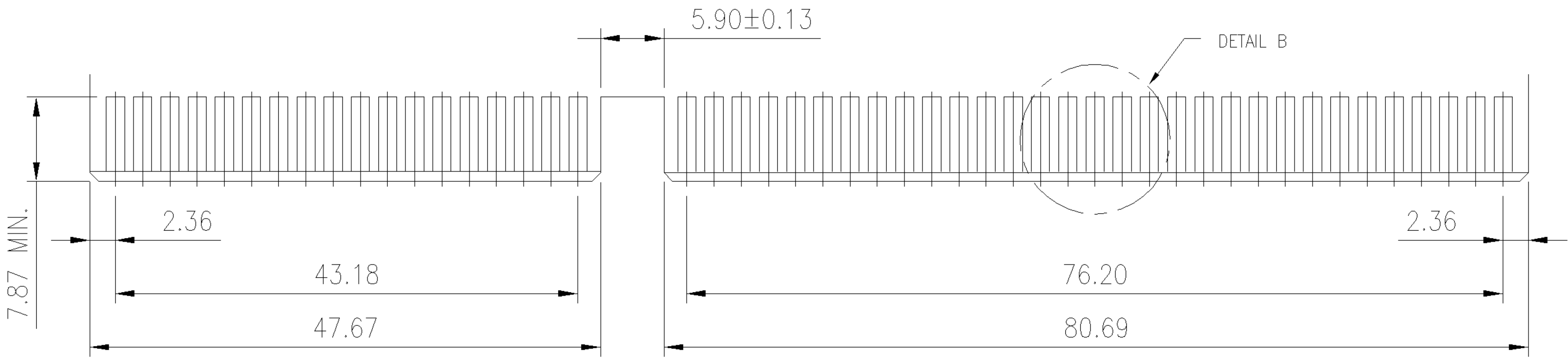
RECOMMENDED MATING COMPONENT BOARD
