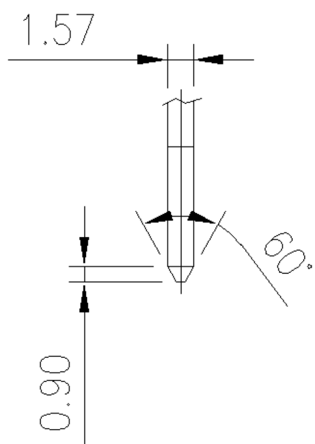
TYPICAL CARD EDGE PROFILE
