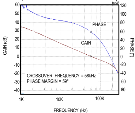
MAX17505 3.3V OUTPUT BODE PLOT (1.7A LOAD CURRENT, FIGURE 4 CIRCUIT)
