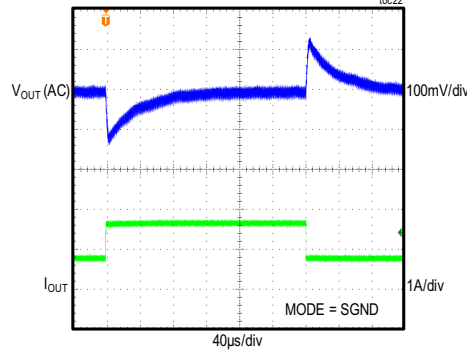
MAX17505 5V OUTPUT LOAD CURRENT STEPPED FROM 0.85A TO 1.7A (PWM MODE, FIGURE 3 CIRCUIT)
