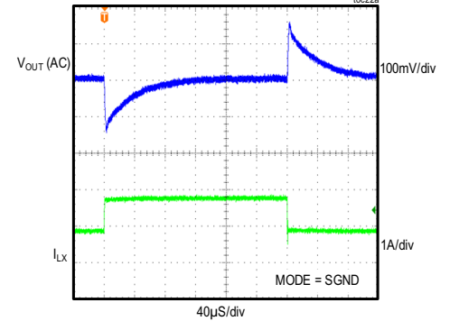
MAX17505S 5V OUTPUT LOAD CURRENT STEPPED FROM 0.85A TO 1A (PWM MODE, FIGURE 5 CIRCUIT)
