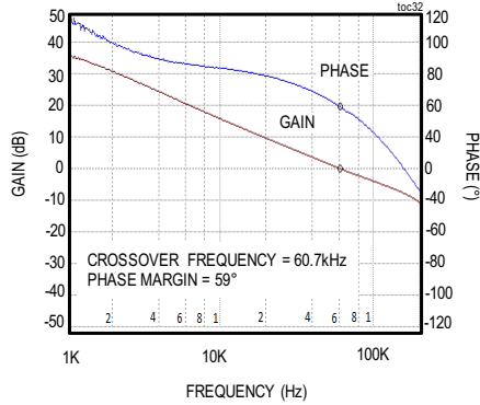
MAX17505 5V OUTPUT BODE PLOT (1.7A LOAD CURRENT, FIGURE 3 CIRCUIT)
