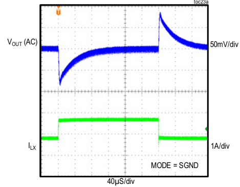
MAX17505S 3.3V OUTPUT LOAD CURRENT STEPPED FROM 0.85A TO 1.7A (PWM MODE, FIGURE 6 CIRCUIT)
