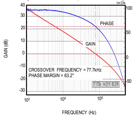
MAX17505S 3.3V OUTPUT BODE PLOT (1.7A LOAD CURRENT, FIGURE 6 CIRCUIT)
