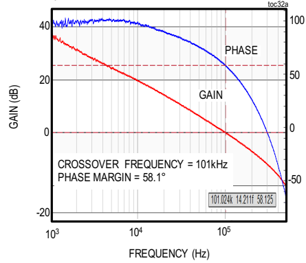
MAX17505S 5V OUTPUT BODE PLOT (1.7A LOAD CURRENT, FIGURE 5 CIRCUIT)
