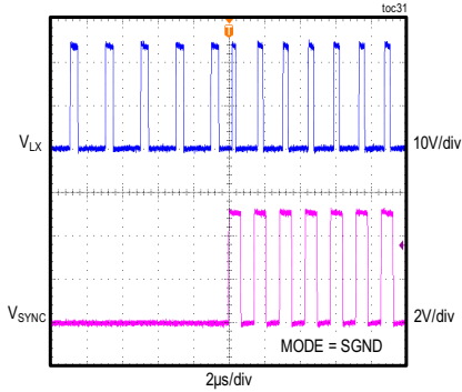
MAX17505 5V OUTPUT APPLICATION OF EXTERNAL CLOCK AT 700kHz (FIGURE 3 CIRCUIT)
