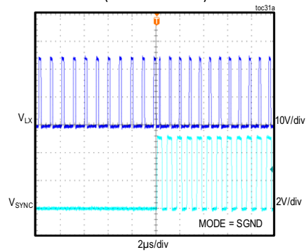
MAX17505S 5V OUTPUT APPLICATION OF EXTERNAL CLOCK AT 1.2MHz (FIGURE 5 CIRCUIT)
