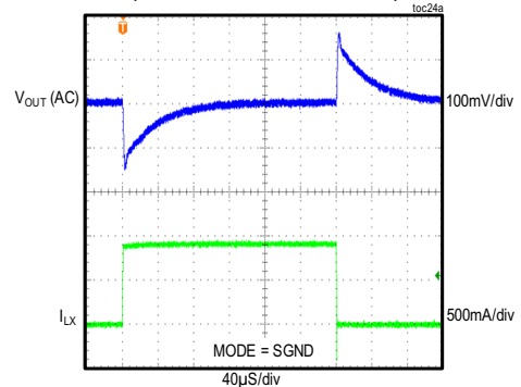
MAX17505S 5V OUTPUT LOAD CURRENT STEPPED FROM NO LOAD TO 0.85A (PWM MODE, FIGURE 5 CIRCUIT)
