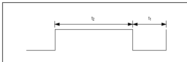
Figure 1. PWM Waveform Timing
