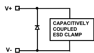
CIRCUIT 4
