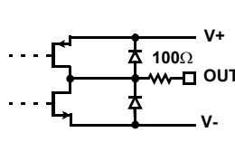
CIRCUIT 3
