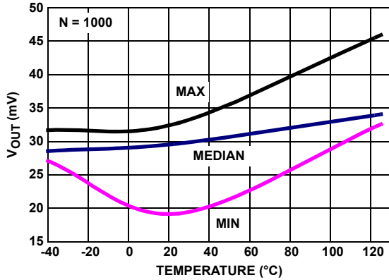
FIGURE 35. ISL28196 V_{OUT} LOW vs TEMPERATURE, V_+ , V_- = \pm 2.5V , R_L = 10k
