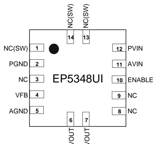
Figure 2: EP5348UI Pin Out Diagram (Top View)
