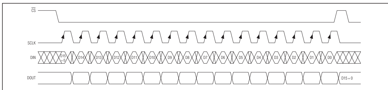
Figure 5. 16-Bit Write Transmission to the MAX7317
