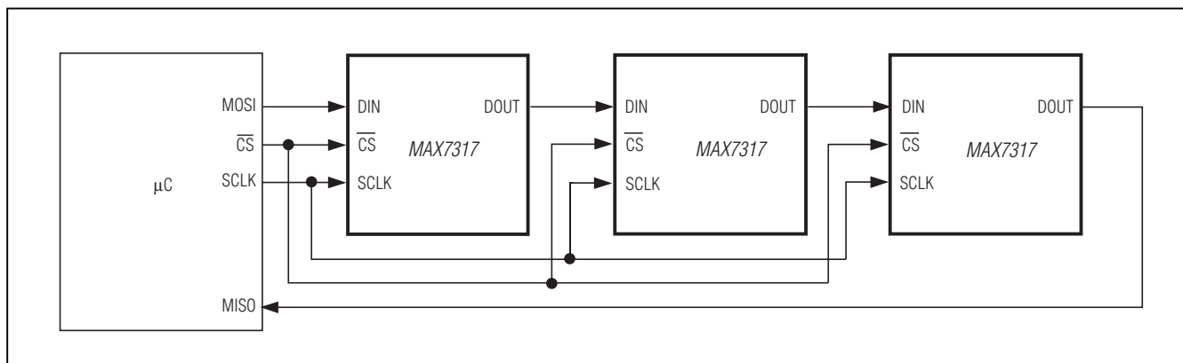
Figure 3. MAX7317 Daisy-Chain Connection
